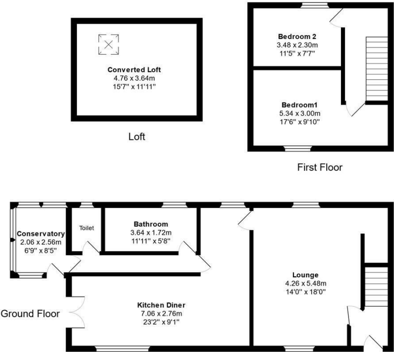
Floor Plans: Greystone Cottage, Allonby Not to Scale: Dimensions and layout for guidance only
